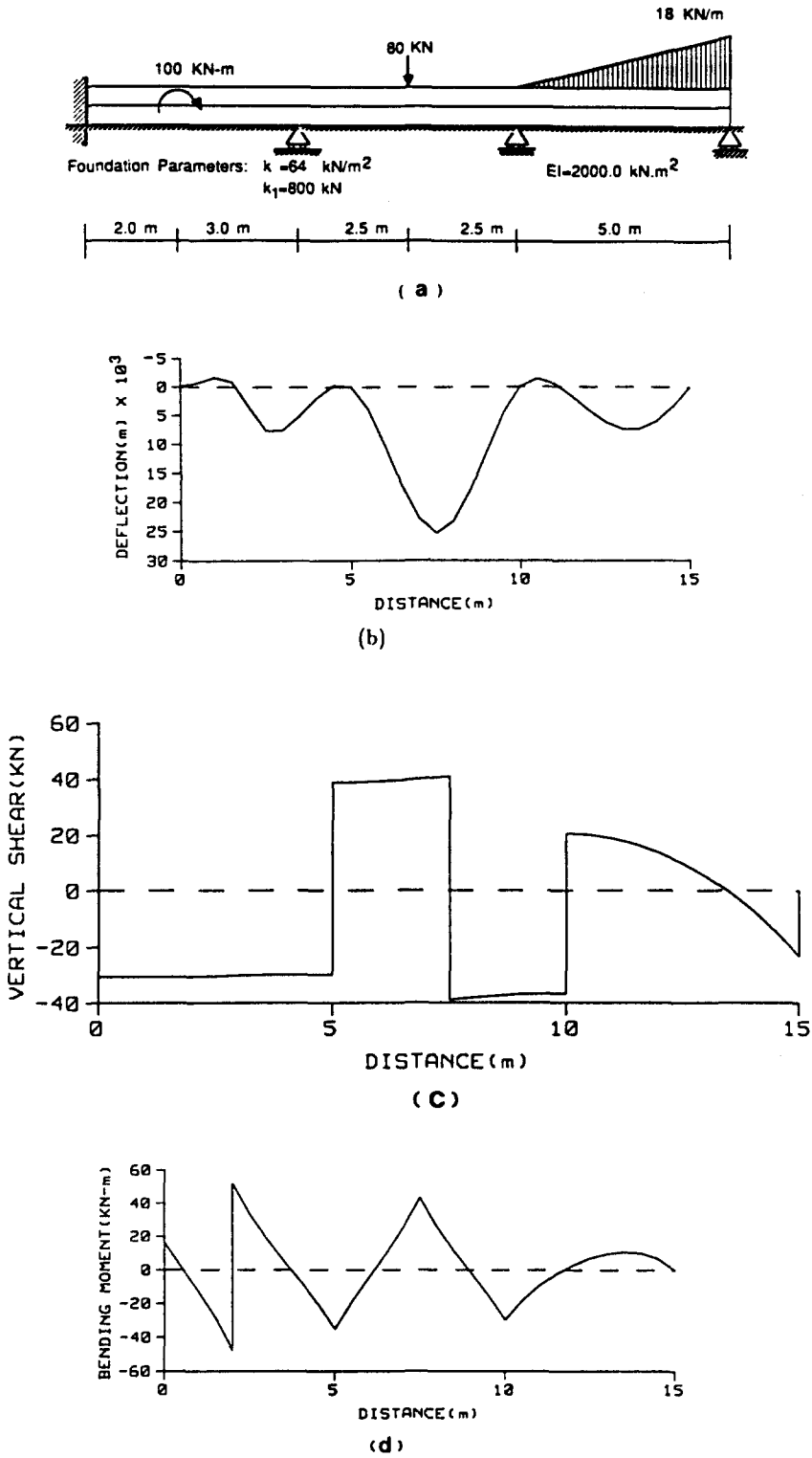
Fig. 6. (a) Continuous beam on two-parameter elastic foundation; (b) deflected shape; (c) vertical shear; (d) bending moment.
